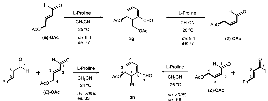
SCHEME 3. Reactions of ( E )-3-Formylallyl Acetate and ( Z )-3-Formylallyl Acetate
