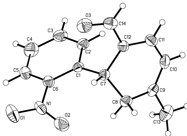
FIGURE 1. ORTEP plot for X-ray crystal structure of 3c .
