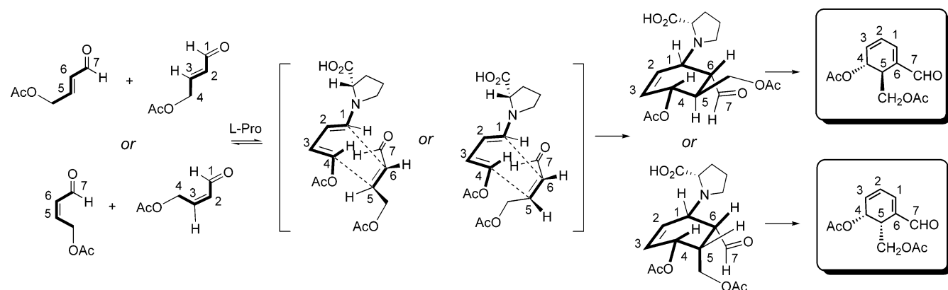
SCHEME 3. Reactions of ( E )-3-Formylallyl Acetate and ( Z )-3-Formylallyl Acetate
