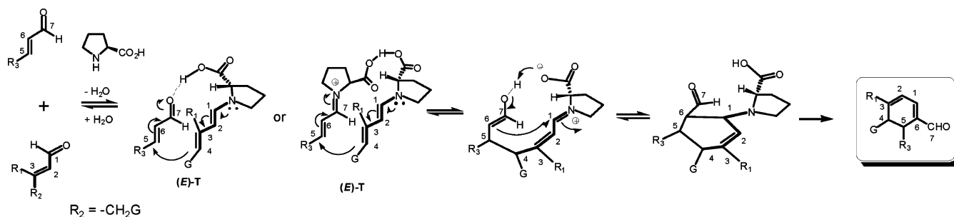
SCHEME 2. Proposed Mechanism for the Formation of [4 + 2] Adduct via Dienamine-Catalyzed Diels–Alder Reaction
